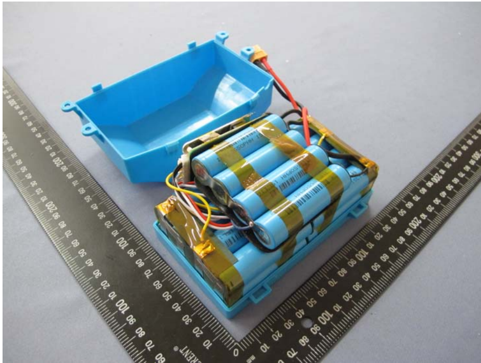
Figure 3 Internal view I of battery pack
